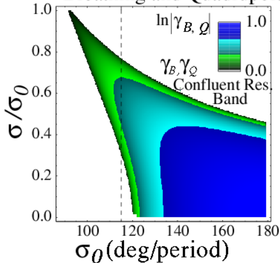
Breathing and Quadrupole Mode Growth Factors, \gamma_B and \gamma_Q
