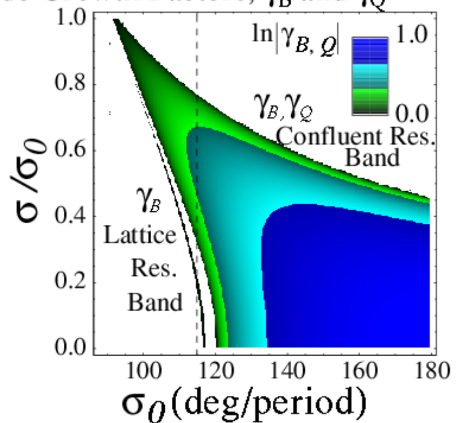
Breathing and Quadrupole Mode Growth Factors, \gamma_B and \gamma_Q
