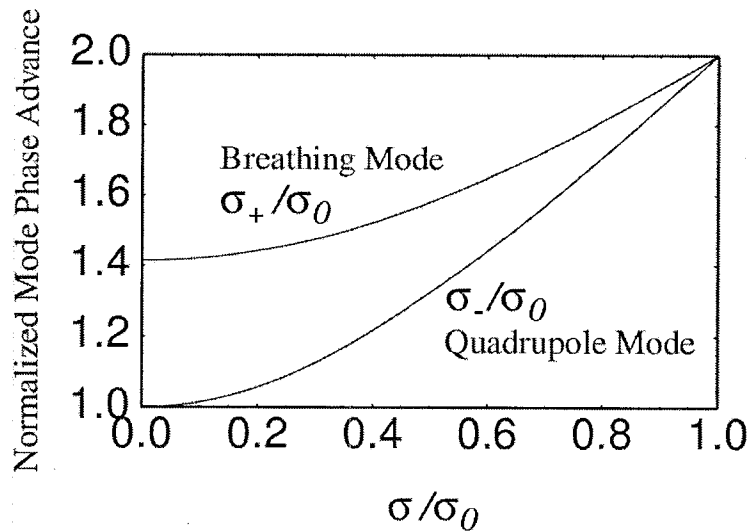
Mode Phase Advances
